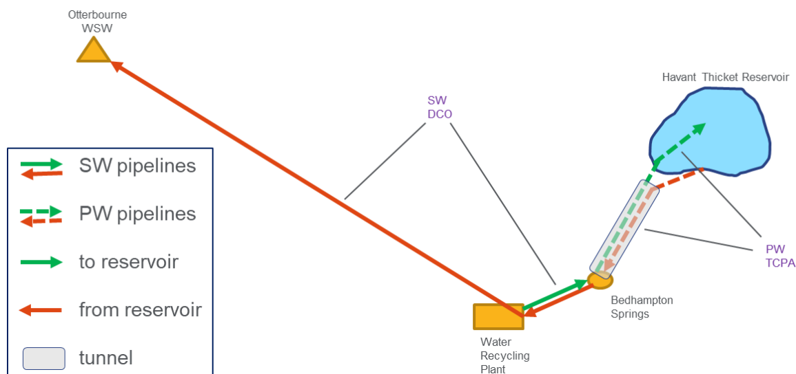
Figure 3: Project utilises Portsmouth Water's twin tunnelled pipelines between Bedhampton Springs and Havant Thicket Reservoir
