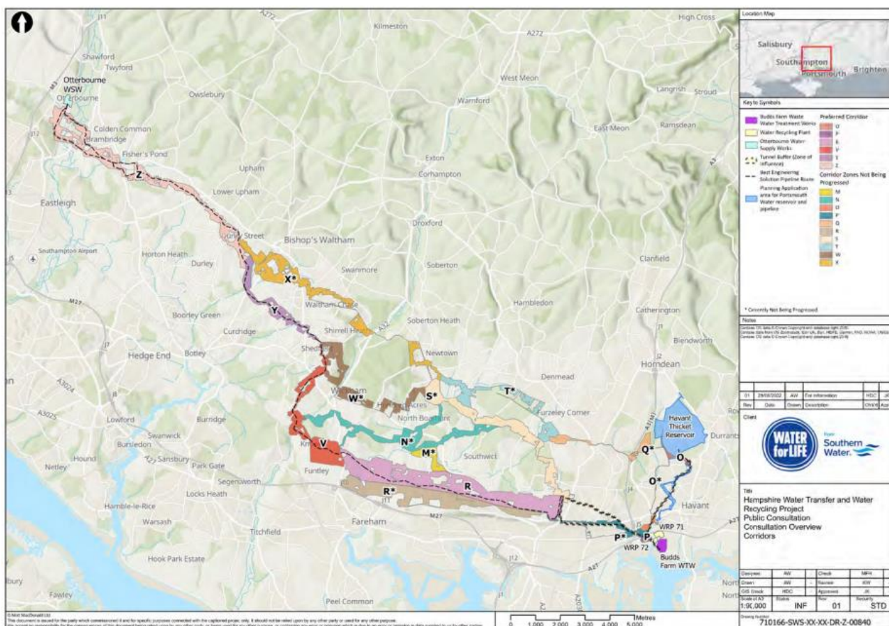
Figure 2. Pipeline corridors consulted on in summer 2022 public consultation
